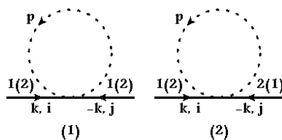
Figure 3. The 2-point fermion diagrams: (1) \Delta\Pi_1 , (2) \Delta\Pi_2 . The fermionic propagator is marked by a dashed line. The numbers indicate the propagator indices; e.g. in (2) there are two contributions coming from G_{12} and G_{21} . External solid lines mark the incoming scalars X^i and X^j , with momenta k and -k respectively.
