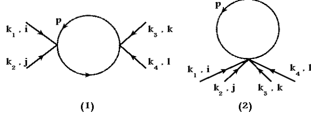
Figure 6. The 4-point scalar diagrams: (1) M_{B1}^4 , (2) M_{B2}^4 .
