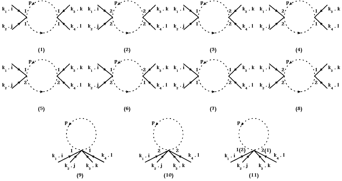
Figure 5. The 4-point fermion diagrams: (1) M_{F1}^4 , (2) M_{F2}^4 , (3) M_{F3}^4 , (4) M_{F4}^4 , (5+6) M_{F5}^4+M_{F6}^4 , (7) M_{F7}^4 , (8) M_{F8}^4 , (9) M_{F9}^4 , (10) M_{F10}^4 , (11) M_{F11}^4 .
