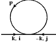
Figure 4. The 2-point scalar diagram \Delta\Pi_3 . Both massive and massless scalars are marked by solid lines.
