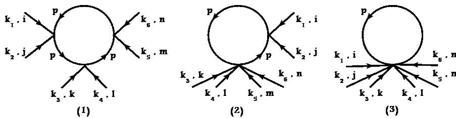
Figure 7. The 6-point scalar diagrams: (1) M_{B1}^6 , (2) M_{B2}^6 , (3) M_{B3}^6 .
